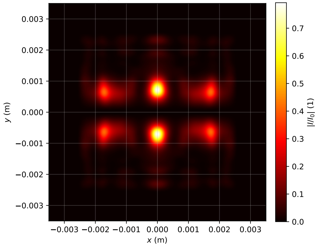
Intensity profile I(x, y, z = 3.503)/I_0 , P_{in}=5.0P_{cr} , artificial time
